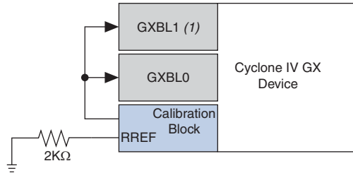
Figure 1-40. Transceiver Calibration Blocks Location and Connection
