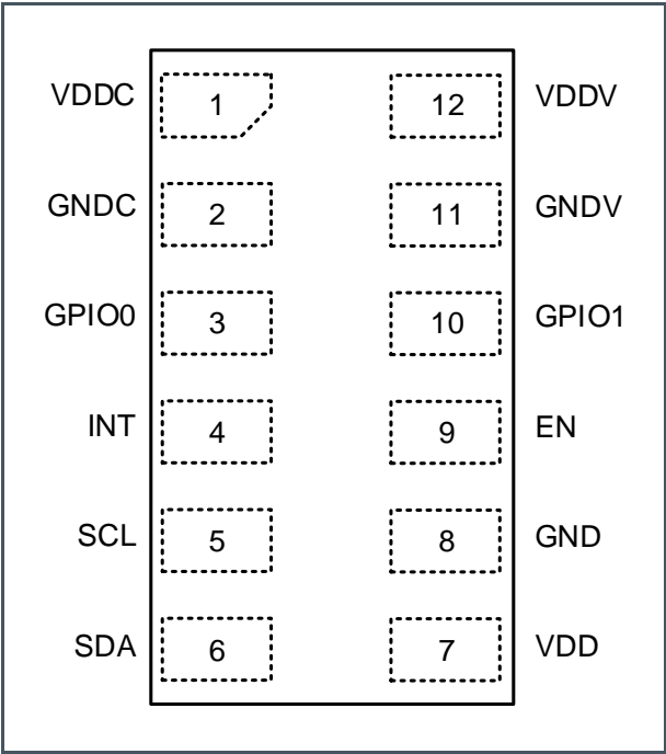
Figure 3: Pin Locations Top Through View (not to scale)
